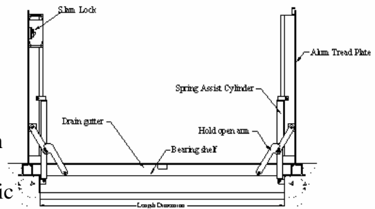
Type "HD" (Double-Leaf Door)
